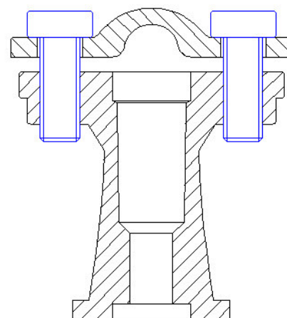
Cross section
