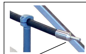
Detail end-connection
