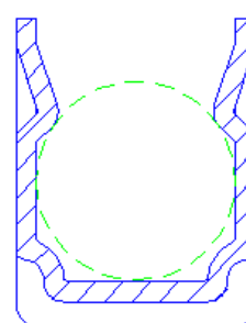
Cross Section
