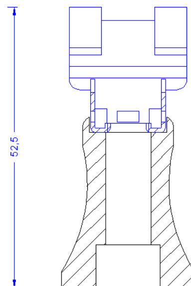
Cross-Section
