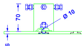
Detail: mounting plate
