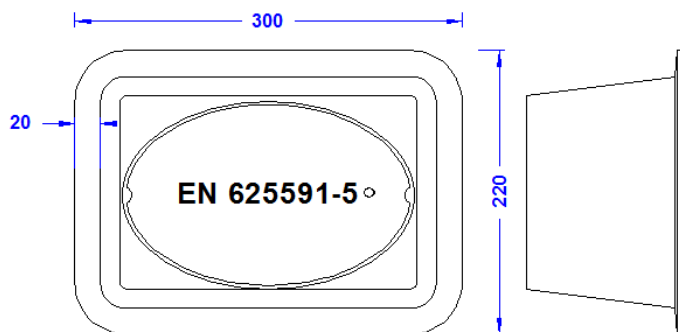
Top with lid
